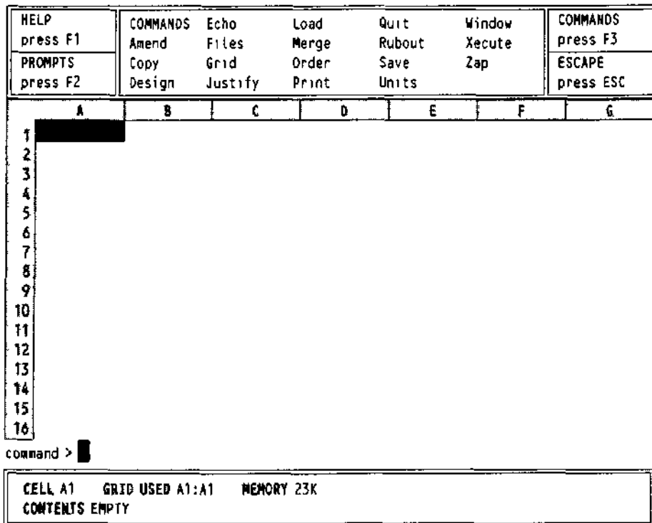
Figure 29 The command menu
